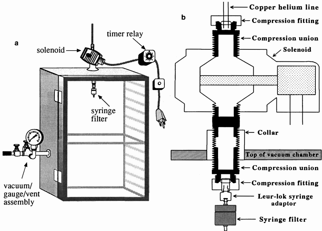
Figure 1. a. Graphic illustration of the Particle Inflow Gun.
